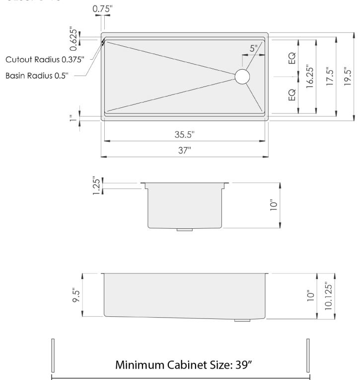
5LS37C-10
